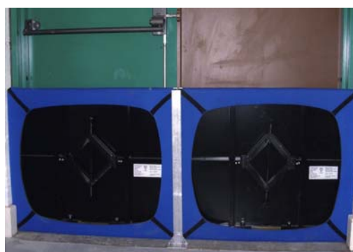
Willowholme Substation – demonstrating how Floodgates can be used to protect emergency exits
